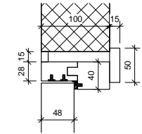
3 Head Detail 1 : 5
