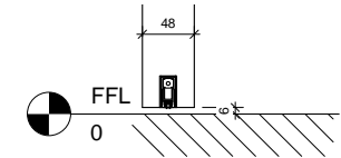
4 Undercut Detail 1 : 5
