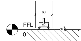
4 Undercut Detail 1 : 5
