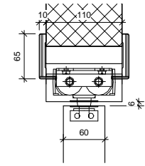
3 Head Detail 1 : 5
