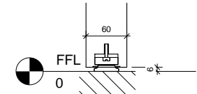
4 Undercut Detail 1 : 5
