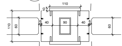
6 Meeting Stile 1 : 5
