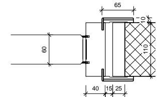
4 Undercut Detail 1 : 5
