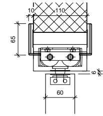
3 Head Detail 1 : 5
